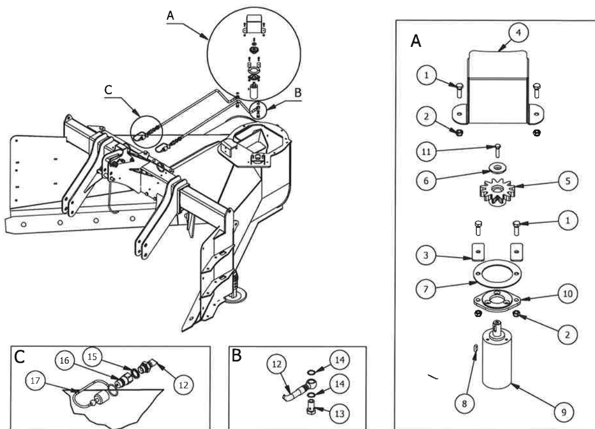
RESERVEDELSLISTE – SPARE PARTS LIST
