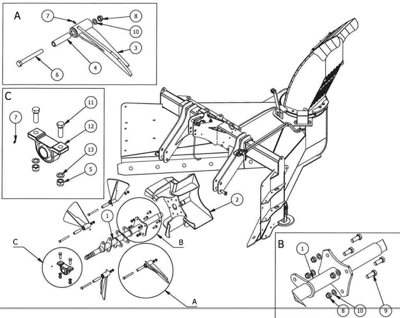
RESERVEDELSLISTE – SPARE PARTS LIST
