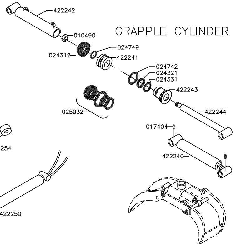
EXTENSION CYLINDER
